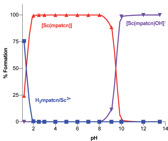
Fig. 4 Complex speciation diagram based on ^1\text{H} NMR data acquired at pH values ranging from 1.15–13.4, connecting curves are drawn between individual points for guidance.
