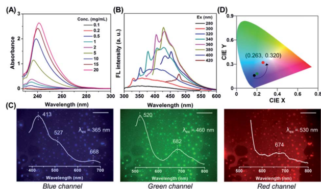
Fig. 2 (A) Absorption spectra of PNVCL at different concentrations in THF. (B) PL spectra of PNVCL recorded at different excitation wavelengths \lambda_{\text{ex}} . Concentration = 20 \text{mg mL}^{-1} in THF. (C) Fluorescence microscopy images of the PNVCL film obtained from the blue (420–460 nm), green (510–550 nm) and red (575–625 nm) emission channels, respectively. Emission spectra of the PNVCL film with different \lambda_{\text{ex}} values are also included in each photograph. Scale bars = 50 \mu\text{m} . (D) The emission regions of fluorescent PNVCL in THF (black dot) and water (green dot) and in the solid state (red dot) assigned in the CIE x,y chromaticity diagram.
