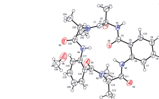
Fig. 2 X-ray crystallographic structure of 1 . 25
