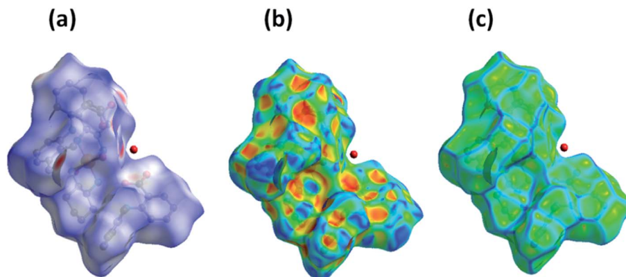
Fig. 3 Hirshfeld surface map representing (a) d_{\text{norm}} , (b) shape index and (c) curviness of complex 1 .
