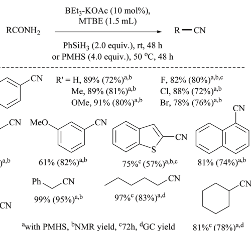
Scheme 48 BEt 3 /base reagent for dehydration.
