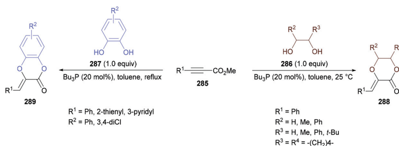
Scheme 72 Phosphine-catalyzed synthesis of 1,4-dioxane-2-ones and 1,4-benzodioxine-2-ones from 1,2-diols and alkyneates.
