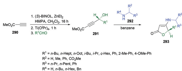
Scheme 73 Asymmetric synthesis of 4-amino-2(5 H )-furanones from alkyneates, aldehydes and amines.
