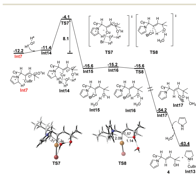
Fig. 3 Free energy profile ( \Delta G in \text{kcal mol}^{-1} ) for \text{H}_2\text{O} -assisted stepwise protodemetalation of Int7 . Bond lengths are given in angstroms.
