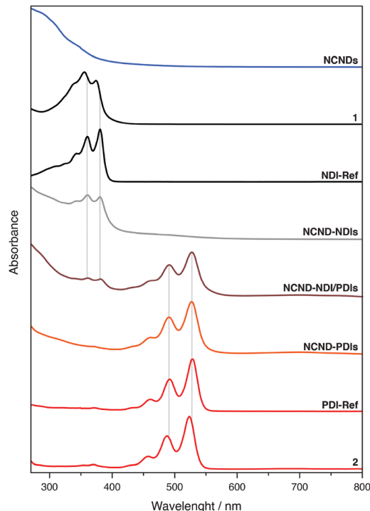
Fig. 4 UV-Vis absorption spectra of rylene diimide precursors ( 1 and 2 ), references (NCND, NDI-Ref, PDI-Ref) and hybrid materials (NCND-NDI, NCND-PDI, NCND-NDI/PDI) in DMF, at room temperature. Vertical lines in grey are guides to help the comparison between the naphthalene and perylene diimide-based materials.
