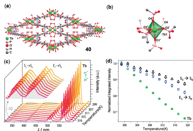
Fig. 32 (a) Crystal packing network and (b) \text{Tb}(\text{III}) octahedral coordination environment of Tb MOF 40 . (c) Temperature-dependent solid-state emission spectral change of 40 in the range of 299\text{--}319\text{ K} ( \lambda_{\text{ex}} = 300\text{ nm} ). (d) Temperature dependence of integrated intensities of different emissions. Reprinted with permission from ref. 142. Copyright 2017 American Chemical Society.
