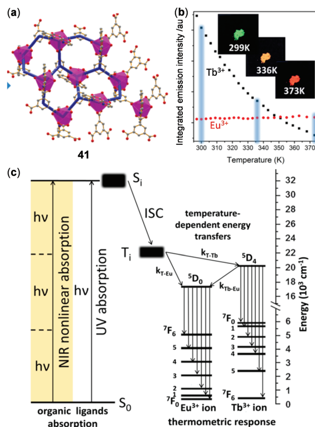
Fig. 33 (a) Honeycomb-like \text{Eu}/\text{Tb} mixed 2D coordination polymer 41 . (b) Plots of the integrated intensity of ^5\text{D}_0 \rightarrow ^7\text{F}_2 of \text{Eu}(\text{III}) (red dots) and ^5\text{D}_4 \rightarrow ^7\text{F}_5 of \text{Tb}(\text{III}) (black dots) f-f emission as a function of temperature (excited at 337\text{ nm} ). Insets: Photographs showing the emission color of 41 at 299 , 336 , and 373\text{ K} , respectively. (c) Energy level diagram highlighting the use of three-photon excitation for effecting the thermometric luminescent response. Reprinted with permission from ref. 145. Copyright 2019 American Chemical Society.
