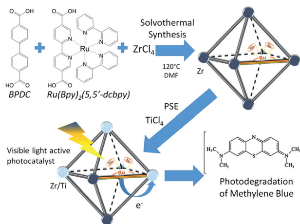
Fig. 14 Schematic processes for preparing a \text{UiO-67-Ru-Ti} MOF and its application. 113 Adapted with permission from ref. 113, © 2017 Elsevier B.V.
