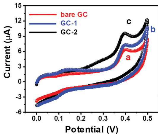
Fig. 7 CV curves of (a) the bare GC, (b) GC-1 and (c) GC-2 in the presence of 250 μM urea in 0.1 M PBS (pH = 7.0) at an applied scan rate of 0.1 V s -1 .
