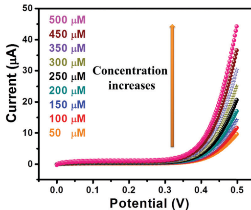
Fig. 9 I - V curves of GC-2 in different concentrations (50–500 μM) of urea in 0.1 M PBS (pH = 7.0).
