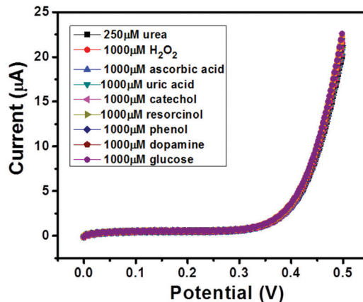
Fig. 11 I - V curves of GC-2 in the presence of urea (250 μM) in 0.1 M PBS (pH = 7.0) with different interfering species (1000 μM).
