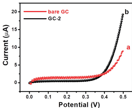
Fig. 8 I - V curves of (a) the bare GC and (b) GC-2 in the presence of 250 μM urea in 0.1 M PBS (pH = 7.0).
