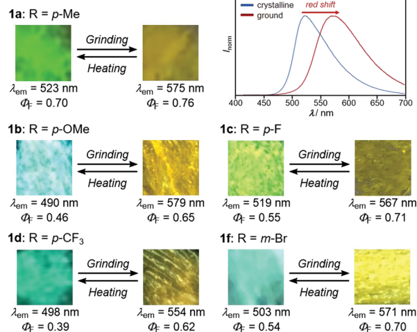
Fig. 7 Photographs and fluorescence spectra for the bathochromically shifted bicolor MCL of 1a-d and 1f excited with UV light ( 365 \text{ nm} ). For the fluorescence spectra for the MCL of 1b-d and 1f , see Fig. S12 (ESI † ).
