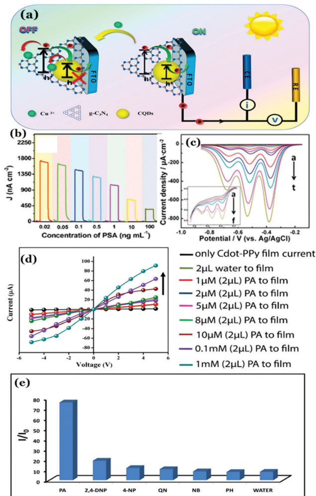
Fig. 15 (a) Mechanism of \text{Cu}^{2+} -quenched photocurrent of Cdots/g- \text{C}_3\text{N}_4 heterostructures. (b) Photocurrent responses of the Cdots/g- \text{C}_3\text{N}_4 sensing platform towards prostate-specific antigen (PSA) with different concentrations. Reprinted with permission from ref. 240. Copyright 2017 American Chemical Society. (c) Differential pulse voltammograms (DPVs) responding to different concentrations of TNT at the CDs/GC electrode. Reprinted with permission from ref. 244. Copyright 2015 American Chemical Society. (d) I - V characteristics of the Cdot-PPy composite film in the presence of different concentrations of picric acid (PA) solutions. (e) The ratios of current flowing through the composite film following addition of 2.0 \mu\text{L} 1.0 mM aqueous solution of different analytes. In the figure PA = picric acid, 2,4-DNP = 2,4-dinitrophenol, 4-NP = 4-nitrophenol, NB = nitrobenzene, PH = phenol, QN = 1,4-benzoquinone, 4-MBA = 4-methoxybenzoic acid. The measurements were made at +5 V. Reprinted with permission from ref. 119. Copyright 2016 American Chemical Society.
