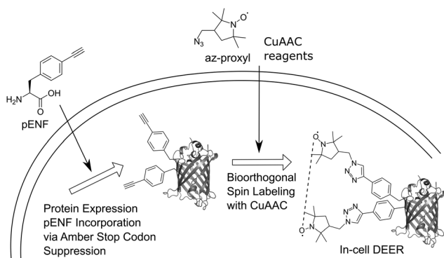
Fig. 1 Schematic overview of the in vivo spin labeling approach via copper-catalyzed [3+2] azide–alkyne cycloaddition followed by in-cell EPR distance determination. The nCaa pENF is incorporated site-specifically into eGFP using amber stop codon suppression. The eGFP-expressing E. coli cells are subjected to CuAAC-based spin labeling and subsequent, DEER distance determination is performed directly inside the cell.
