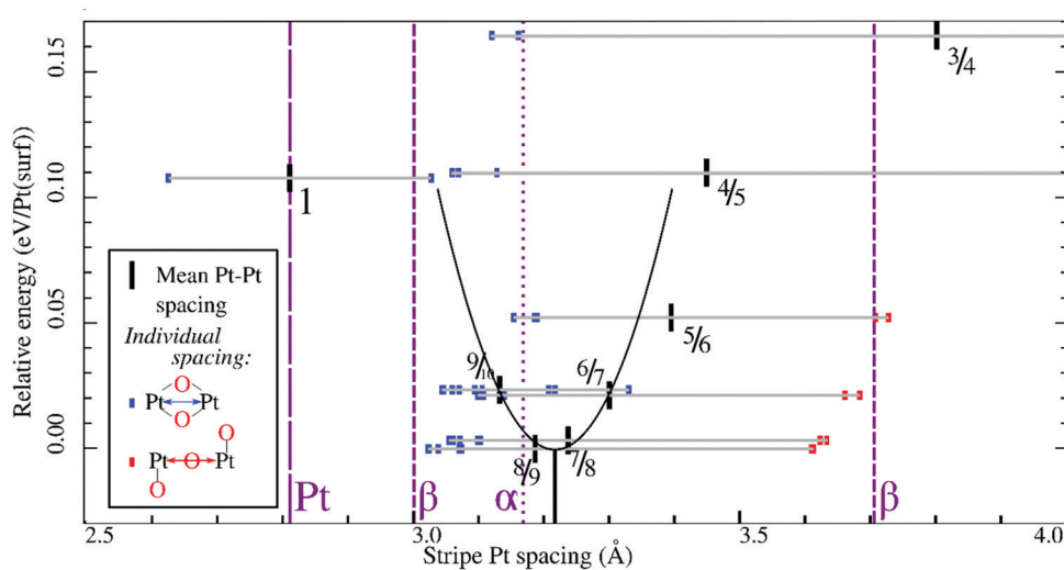
Fig. 4 Relative stripe formation energies (per surface platinum atom, without vibrational contribution to the energy) versus individual Pt–Pt distances (in the stripe) and mean spacings, including a quadratic fit of mean spacings near the energy minimum (marked by a descender from the apex of the parabola) and bulk Pt–Pt spacings for Pt, \alpha -PtO 2 and \beta -PtO 2 ; legend in inset.
