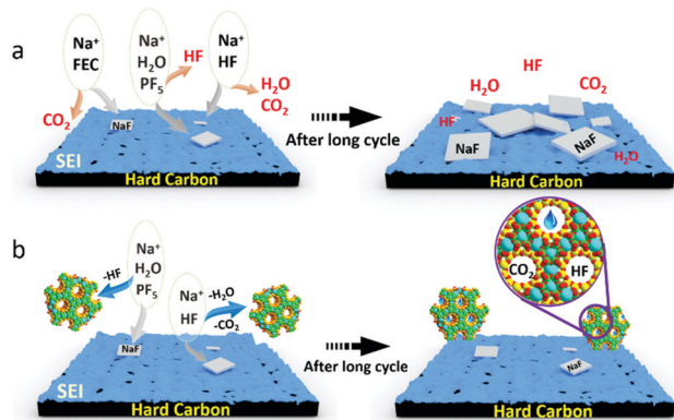
Fig. 4 Schematic diagram of the proposed mechanism of FEC (a) and NZeo (b) electrolyte additives in the long term cycling process as described with eqn (1)–(4) and SEM images (ESI†).
