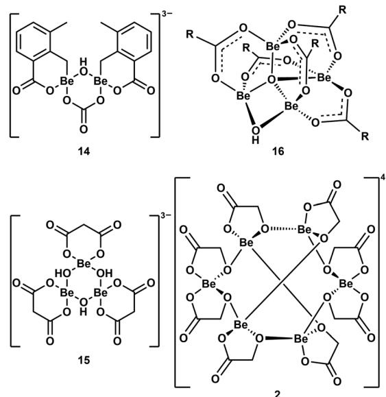
Fig. 8 Multinuclear beryllium compounds with bio-relevant ligands, which all contain six- or eight-membered beryllium heterocycles ( R = 2\text{-F-C}_6\text{H}_4 ). 39,41,57,58
