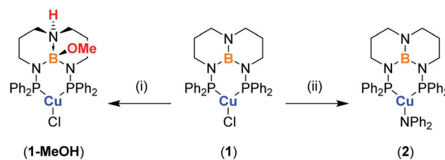
Scheme 1 Structure of ( Ph TBDPhos)CuCl ( 1 ) and synthesis of 1-MeOH and 2 . (i) Excess MeOH at RT. (ii) Addition of 1 eq. of HNPh 2 and KN(SiMe 3 ) 2 in toluene at -78 °C.
