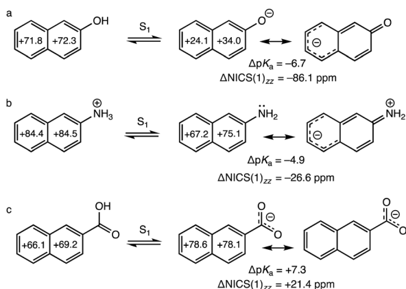
Fig. 1 Computed NICS(1) zz and \Delta NICS(1) zz (sum of NICS(1) zz values of the conjugate base minus that of the acid (in ppm) values for the S_1 states of the acid and conjugate base at CASSCF(12,12)/6-311+G(d,p), for (a) 2-naphthol, (b) 2-naphthylammonium, and (c) 2-naphthoic acid. Negative \Delta NICS(1) zz values indicate antiaromaticity relief, and positive values indicate antiaromaticity gain, upon formation of the excited conjugate base. Experimental \Delta pK_a values are included for reference.
