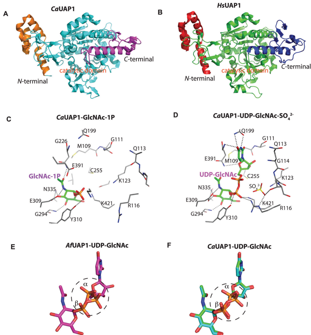
Fig. 3 Comparison of AfuUAP1 with other UAP1s. (A) Overall structure of CaUAP1. Coloured in orange, cyan and purple are the N-terminal, catalytic and C-terminal domains, respectively. (B) Overall structure of HsUAP1. Coloured in red, green and blue are the N-terminal, catalytic and C-terminal domains, respectively. (C) Active site of CaUAP1 with GlcNAc-1P bound. Active site residues are shown in sticks. Hydrogen bond interactions are shown as black dashes. (D) Active site of CaUAP1 with UDP-GlcNAc-SO 4 2- bound. Active site residues are shown in sticks. Hydrogen bond interactions are shown as black dashes. SO 4 2- is shown as sticks. (E) Stick representation of UDP-GlcNAc in the AfuUAP1-UDP-GlcNAc-Pi-Mg 2+ ternary complex, showing the observed dual conformation around the \alpha -phosphate. (F) Superposition of UDP-GlcNAc from the CaUAP1-UDP-GlcNAc product complex (PDB: 2yqs, blue) with UDP-GlcNAc from the CaUAP1-UDP-GlcNAc reaction-completed product complex (PDB: 2yqj, green). This superposition recapitulates the dual conformation observed in the AfuUAP1-UDP-GlcNAc-Pi-Mg 2+ complex.
