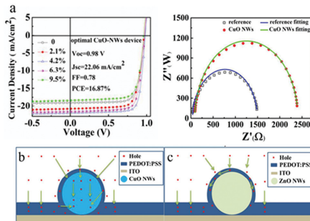
Fig. 20 (a) J - V curves of PSCs with different coverage of CuO NWs, under 100 \text{mW cm}^{-2} illumination (AM 1.5G) and Nyquist plots of PSCs without and with the optimal coverage of CuO-NWs in the dark and (b) schematic illustration of hole transport with CuO NWs. 129
