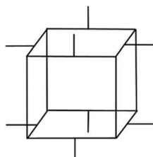
Isocube
