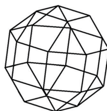
Rhombicuboctahedron
