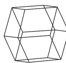
Rhombic Dodecahedron
