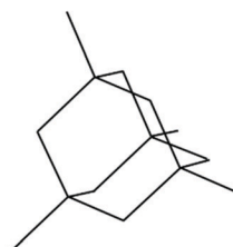
Diamond
