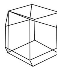
Rhombic trapezoidal-dodecahedron
