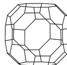
Truncated Cuboctahedron
