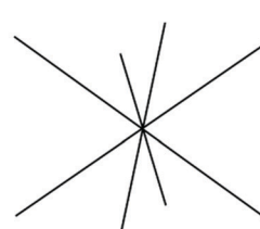
Body-Centered Cubic
