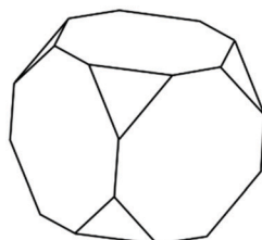
Truncated cube
