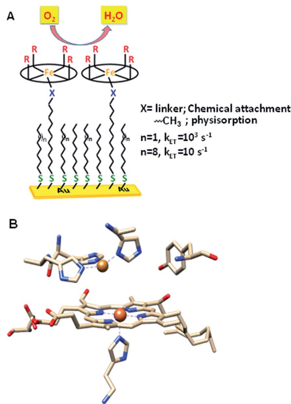
Fig. 1 (A) Heterogeneous electrochemical construct (the oval ring represents the porphyrin ligand); (B) binuclear active site of CcO (PDB ID: 1OCC). 9
