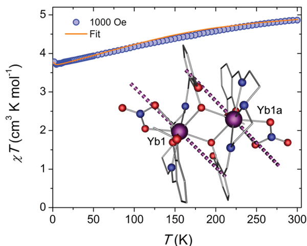
Fig. 1 Temperature dependence of the \chi T product at 1000 Oe (blue spheres), and comparison with the calculated magnetic susceptibility assuming J = 0.005 cm -1 (solid orange line). The inset displays the molecular structure of the {Yb 2 } complex along with the orientation of the main magnetic axis in the ground state of the Yb III ions as shown in the purple dashed lines. Colour code: purple (Yb), red (O), blue (N); while all unfilled grey vertices represent carbon atoms.
