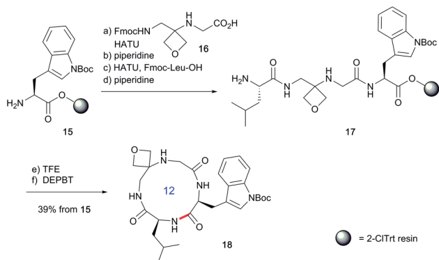
Scheme 4 Synthesis of oxetane modified cyclic peptide 18 by SPPS. Reaction conditions: (a) 16 (2 equiv.), HATU (1.9 equiv.), i Pr 2 EtN (4.0 equiv.), DMF, 2–4 h, double coupling; (b) 20% piperidine, DMF, 20 min; (c) Fmoc-Leu-OH (5.0 equiv.), HATU (4.9 equiv.), i Pr 2 EtN (10 equiv.), DMF, 1 h; (d) 20% piperidine, DMF, 20 min; (e) TFE/CH 2 Cl 2 (1 : 4), 3 × 1 h; (f) DEPBT (2.0 equiv.), i Pr 2 EtN (2.0 equiv.), DMF (0.001 M), 64 h.
