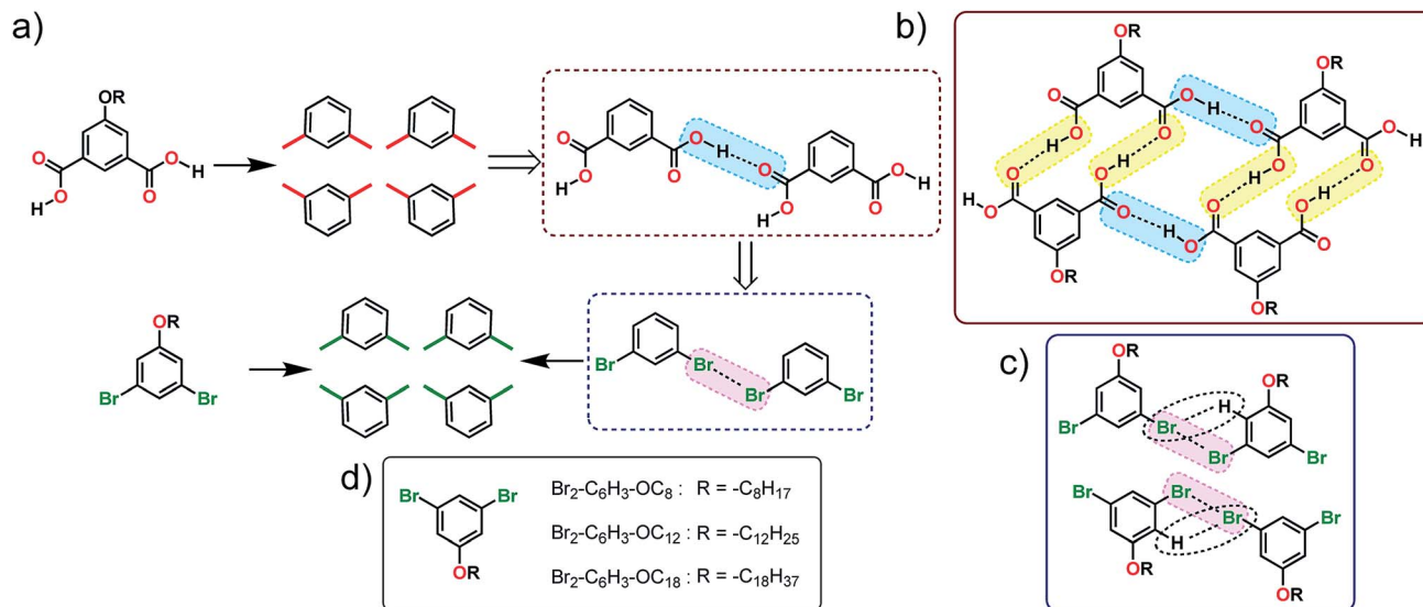
Fig. 1 (a) Schematic showing how the H-bonding/X-bonding analogy can be used in a retrosynthetic approach. The hydrogen bonded O–H⋯O synthon is highlighted in blue while halogen bonded Br⋯Br synthon is highlighted in pink. (b and c) Schematics showing the outcome of self-assembly for alkoxy-substituted isophthalic acid derivatives 17–19 and the corresponding dibromophenyl derivatives (this work), respectively. The inter-row dimeric H-bonds are highlighted in yellow. We note that alkoxy isophthalic acids with relatively short alkoxy chains form 6 membered cyclic hexagonal structures both in 3D 20 as well as in 2D. 17 (d) Molecular structures of the 1,3-dibromo-5-alkoxybenzene derivatives.
