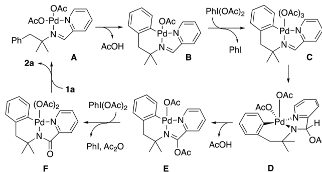
Scheme 8 Indolines formation.
