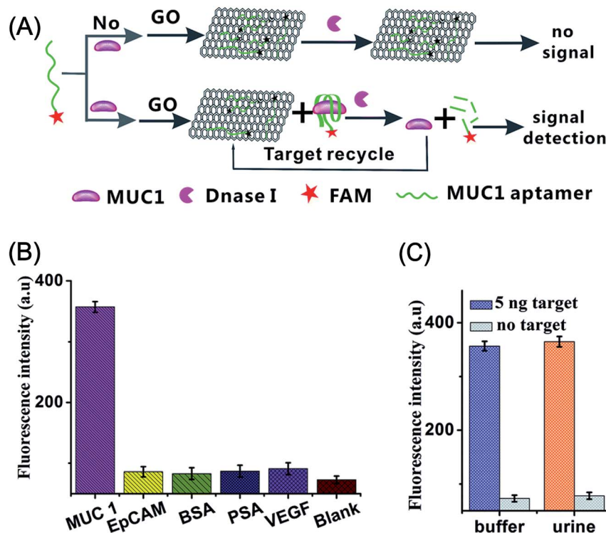
Fig. 775 (A) Schematic representation of a fluorescent aptasensor assay based on GO-probe for detecting mucin 1 protein (MUC1) (5'-FAM-CCCGTCTTCCAGACAAGAGTGCAGGG-3') by using deoxyribonuclease I (DNase I)-mediated target cyclic amplification. The formation of GO-probe/MUC1 complex results in the fluorescence signal detection. (B) Fluorescence intensity of the GO-based aptasensor in the presence of MUC1 (5 ng mL -1 ), epithelial cell adhesion molecule (EpCAM) (50 ng mL -1 ), serum albumin (BSA) (50 ng mL -1 ), prostate-specific antigen (PSA) (50 ng mL -1 ), vascular endothelial growth factor (VEGF) (50 ng mL -1 ), and blank, respectively. (C) Fluorescence intensity of the GO-based aptasensor for detection of MUC1 protein in buffer and blank biological samples of human urine, saliva and serum. Reprinted with permission from ref. 775, J. Zhang, F. Ran, W. Zhou, B. Shang, F. Yu, L. Wu, W. Hu, X. He and Q. Chen, Ultrasensitive fluorescent aptasensor for MUC1 detection based on deoxyribonuclease I-aided target recycling signal amplification, RSC Adv. , 2018, 8, 32009–32015. Copyright© The Royal Society of Chemistry.
