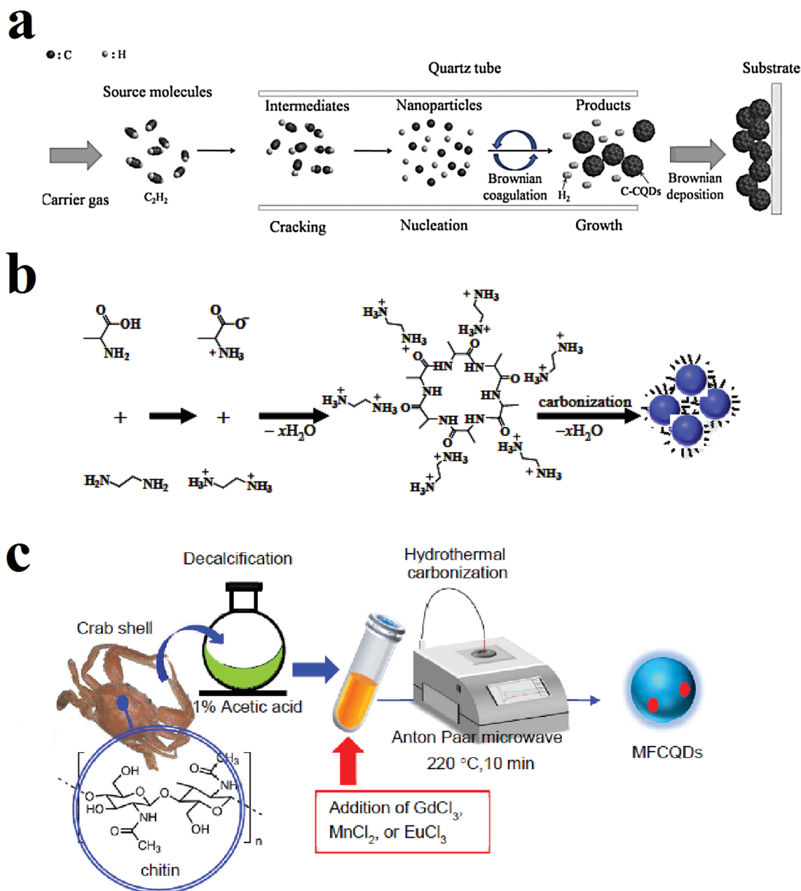
Fig. 2 (a) Synthesis of QDs through CVD method using C_2H_2 as the carbon source, reprinted with permission from ref. 47, copyright 2016 Elsevier Ltd., (b) synthesis of the QDs through the hydrothermal method using alanine and ethylenediamine, reprinted with permission from ref. 66, copyright 2015 Elsevier Ltd., (c) microwave-assisted pyrolysis synthesis of magnetofluorescent QDs from crab shell, reprinted with permission from ref. 81, copyright 2017 American Chemical Society.
