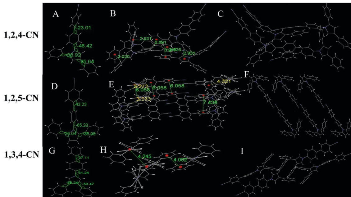
Fig. 4 (A) Molecular structure, (B) interaction distances of C-H \cdots \pi interactions and (C) stacking image of 1,2,4-CN. (D) Molecular structure, (E) interaction distances of C-H \cdots \pi interactions and (F) stacking image of 1,2,5-CN. (G) Molecular structure, (H) interaction distances of face-to-face phenyl rings and (I) stacking image of 1,3,4-CN. Gray color corresponds to carbon, white to hydrogen and blue to nitrogen.
