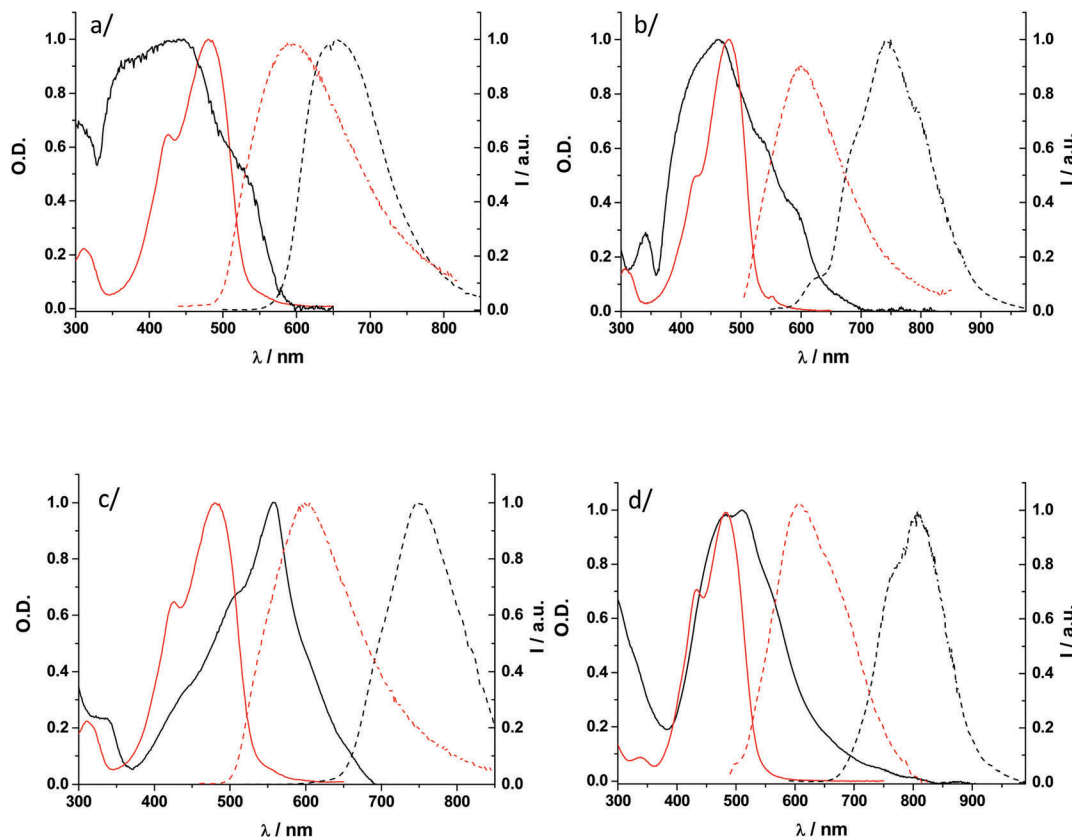
Fig. 4 UV-visible absorption spectra of thin films (—) and solutions in DCM ( - - - ), and fluorescence spectra of powder samples ( ···· ) and solutions in DCM ( - · - · ) for (a) F-F; (b) Cl-Cl; (c) Br-Br and (d) I-I.
