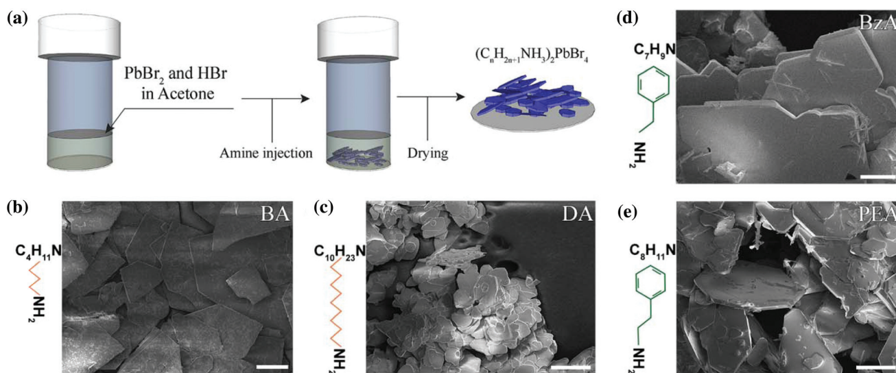
Fig. 1 (a) Schematic diagram of the facile fabrication process of the layered perovskite by injecting a primary amine to a mixture of PbBr 2 in HBr and acetone. (b–e) SEM images of the produced platelets when using short and long aliphatic molecules, such as butylammonium (BA) (b) and decylammonium (DA) (c), and aromatic ones as benzylammonium (BzA) (d) and phenethylammonium (PEA) (e). Scale bars: 100 μm.
