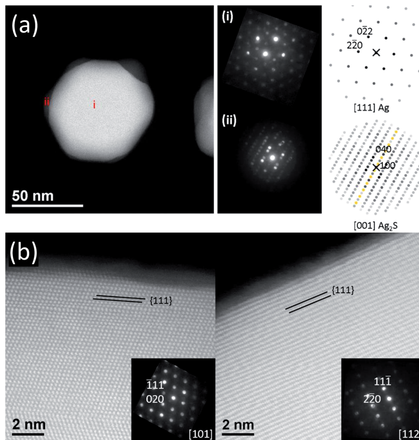
Fig. 3 (a) NBED diffraction patterns from a Ag 2 S/Ag particle after 8 min identify the phase as (i) Ag (space group 225, Fm3m ) and (ii) Ag 2 S (space group 14, P2 1 /c ). Note in (i) forbidden reflections are present due to planar defects. The NBED patterns have been rotated to correspond to the orientation of the real space image and a nonlinear histogram adjustment was made to highlight the presence of weak features. Simulated diffraction patterns accompany the NBED patterns. (b) TEM Images of passivated surfaces. {111} surfaces after 24 h have only a thin Ag 2 S layer present. NBED patterns (inset) have been rotated to correspond to the orientation of the real space image and a nonlinear histogram adjustment was made to highlight the presence of weak features.
