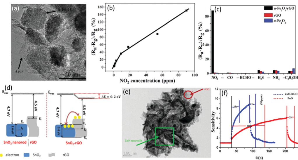
Fig. 23 (a) TEM image of the \alpha -Fe 2 O 3 /rGO composite; (b) response values of the sensor based on \alpha -Fe 2 O 3 /rGO at different NO 2 concentrations; (c) response histogram of the sensor to different gases. 342 Copyright 2014, Royal Society of Chemistry. (d) Band gap diagrams of SnO 2 -nanorods/reduced graphene oxide nanostructures before and after combination. 347 Copyright 2017, Elsevier. (e) TEM image of the ZnO/rGO composite; (f) response/recovery curves to 50 ppm NO 2 of the sensor based on a-ZnO/rGO or ZnO. 135 Copyright 2017, Elsevier.
