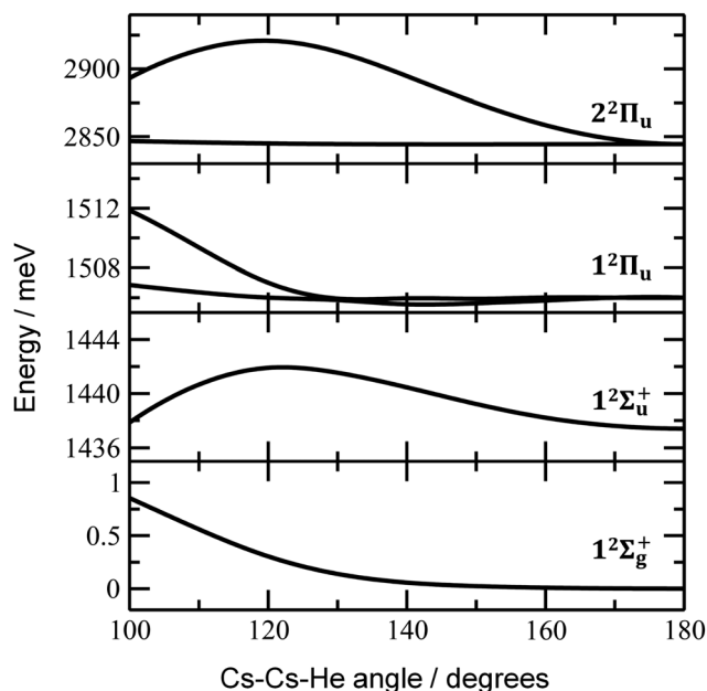
Fig. 3 Dependence of ground state and excited state energies in \text{Cs}_2\text{He}^n on the Cs–Cs–He angle. Calculated at the EOM-CCSD/def2QZVPPD level of theory with ground-state structures optimized at the CCSD/def2QZVP(Cs), def2TZVP(He) level with a constrained Cs–Cs–He angle. Spin–orbit effects were neglected.
