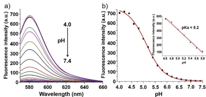
Fig. 15 (a) Change in the fluorescence spectra of probe 12 (1 \mu\text{M} ) in aqueous solution containing DMSO (B–R buffer : DMSO = 95 : 5, v/v) with decreasing pH from 7.4 to 4.0 ( \lambda_{\text{ex}} = 560 nm). (b) Sigmoidal fitting of the pH-dependent fluorescence intensity at 580 nm. Inset: The good linearity in the pH range of 4.6–5.8. Copyright 2015 Elsevier.
