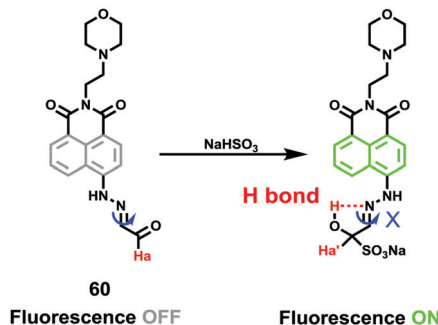
Scheme 46 Fluorescent probe 60 for SO 2 .
