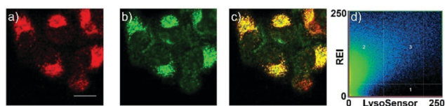
Fig. 16 Confocal fluorescence imaging of living HeLa cells co-stained with probe 12 (5 \mu\text{M} ) and LysoSensor Green (1 \mu\text{M} ) for 1 h. (a) Red emission from probe 12 ; (b) green emission from LysoSensor Green; (c) overlay of (a) and (b); areas of co-localization appeared in yellow; (d) the correlation of LysoSensor Green and probe 12 intensities. Copyright 2015 Elsevier.
