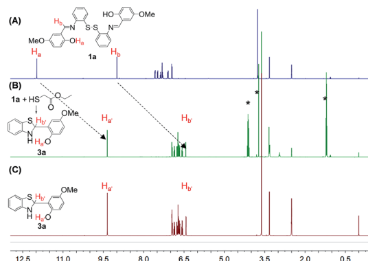
Fig. 1 The 1 H NMR spectra of (A) 1a , (B) “ 1a + ethyl thio-glycolate”, and (C) purified 3a (* represents diethyl 2,2'-disulfanediyldiacetate).
