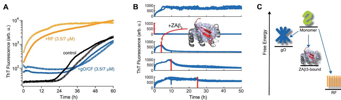
Fig. 3 Metastability and RF seeding incompetence of gO/CFs. (A) HewL RF kinetics below the COC ( 38 \mu\text{M} hewL, 400 \text{ mM} NaCl) without seeding (black), or after seeding with isolated gO/CFs (blue) or RFs (orange) at either 3.5 or 7 \mu\text{M} each, and incubated at \text{pH } 2 , T = 52 \text{ }^\circ\text{C} . (B) ThT-detected dissociation of pre-assembled dimA \beta upon addition of the binding protein ZAB3 (grey), which sequesters monomeric dimA \beta in a \beta -hairpin conformation (red, see ref. 65 and 67). The complex is shown in ribbon representation, hydrophobic side chains of ZAB3 in direct contact with the A \beta 40 \beta -hairpin are shown as spheres (Protein Data Bank entry 2OTK). The assembly of 6 \mu\text{M} dimA \beta was monitored by ThT fluorescence, with addition of 14 \mu\text{M} ZAB3 at different time points, indicated by red lines. Addition of ZAB3 during the gO/CF formation-dominated time regime results in nearly complete loss of ThT fluorescence, while ZAB3 addition during the RF-dominated time regime leads to a progressive decrease in the amplitude of the fluorescence drop. (C) Energy diagram illustrating the order of thermodynamic stability of different states of A \beta , above the COC and under the present experimental conditions.
