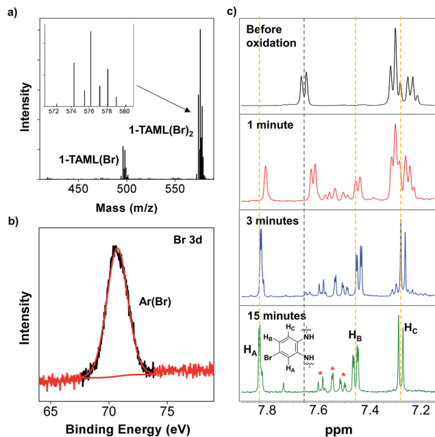
Fig. 3 Characterisation data of 1\text{-TAML}(\text{Br})_n generated from the reaction involving 1 , (\text{ArMe})_3\text{N}^+ (4 eq.), and tetraethylammonium bromide (TEABr, 10 eq.). (a) Negative-ion ESI-MS of the crude reaction mixture 30 minutes after the addition of the (\text{ArMe})_3\text{N}^+ oxidant. The assigned intermediates are labelled. (b) Br 3d XPS data of 1\text{-TAML}(\text{Br})_n . The fit (red, binding energy = 70.7 eV) represents the component completely attributable to aryl bromide. (c) ^1\text{H} NMR spectra of deligated aliquots of the reaction mixture, withdrawn at time intervals 1 (red), 3 (blue), and 15 (green) minutes after the addition of the (\text{ArMe})_3\text{N}^+ oxidant. The spectrum of the TAML before oxidation is shown in black. The dashed lines highlight the characteristic ^1\text{H} NMR signals from the TAML (grey) and the proposed 1\text{-TAML}(\text{Br})_2 (orange). The ^1\text{H} NMR signals (labelled \text{H}_A , \text{H}_B , and \text{H}_C ) are proposed to arise from the major 1\text{-TAML}(\text{Br})_2 isomeric product, while the remaining signals (*) likely originate from another isomer of 1\text{-TAML}(\text{Br})_2 with Br substitution at a different position of the aryl ring.
