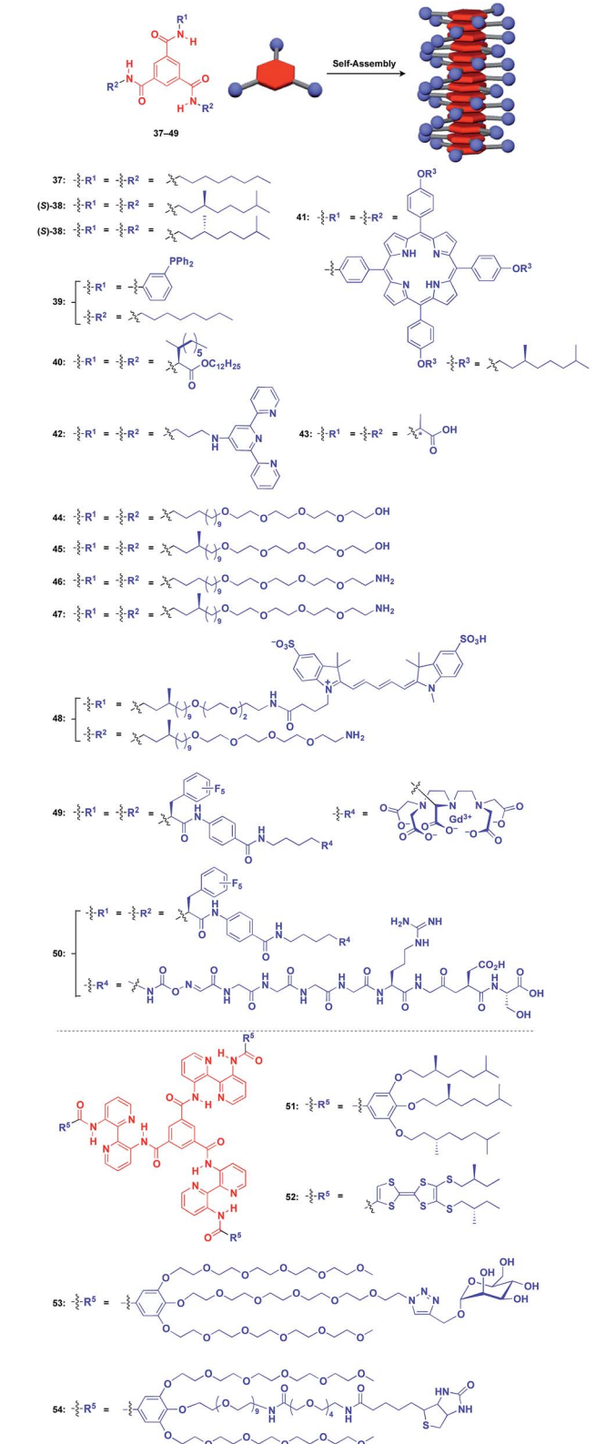
Fig. 9 Schematic structures of BTA-( 37 – 49 ) and extended BTA-based ( 50 – 54 ) helical 1D supramolecular scaffolds (red), and examples of functional molecular units (blue) assembled with the scaffolds.
