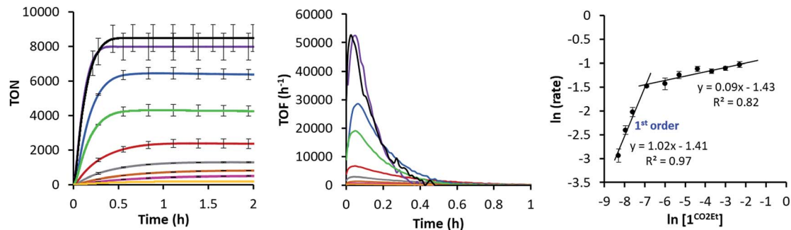
Fig. 5 (Left) Dependence of the H 2 evolution with the concentration of 1 CO 2 Et (100 μM, yellow; 50 μM, pink; 25 μM, orange; 12.5 μM, grey; 5 μM, red; 2.5 μM, green; 1 μM, blue; 0.5 μM, purple; 0.25 μM, black). (Middle) On-line H 2 evolved traces and rates vs. time at different concentrations of 1 CO 2 Et (0.25–100 μM). Conditions: PS Ir + (150 μM) in CH 3 CN : H 2 O : Et 3 N (4 : 6:0.2 mL) irradiated (λ = 447 nm) at 25 °C. (Right) Logarithmic plot of catalytic rate as a function of 1 CO 2 Et concentration.
