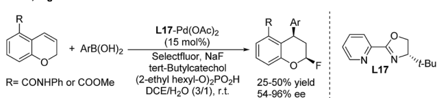
Scheme 13 Pd-catalyzed enantioselective 1,3-arylation of chromenes.
