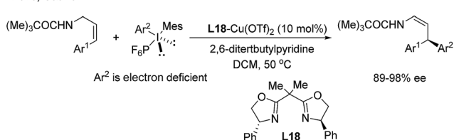
Scheme 14 Cu/BOX-catalyzed enantioselective electrophilic arylation of allylic amides.
