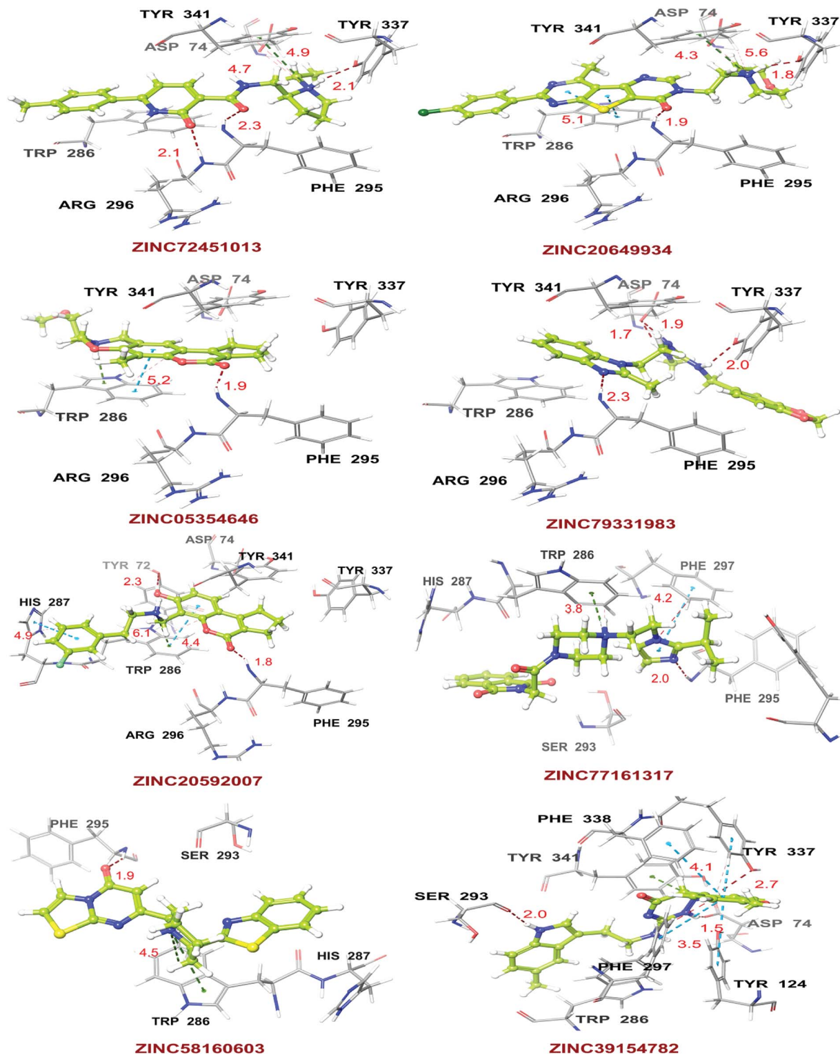
Fig. 6 Docking poses of ZINC72451013, ZINC20649934, ZINC05354646, ZINC79331983, ZINC20592007, ZINC77161317, ZINC58160603, and ZINC39154782 with AChE crystal structure; hits represented in yellowish green, residues in gray, H-bond in red, pi-cationic interaction in green and pi-pi stacking in cyan color.
