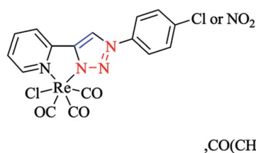
Scheme 27 Structure of the [(C_{13}H_9N_5O_2)ReCO_3Cl (or NO_2 )]· CH_3 · COCH_3 complex.
