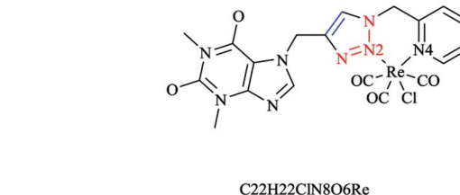
Scheme 28 Structures of the C_{17.25}H_{13}ClN_4O_{3.25}Re , C_{19}H_{18}ClN_4O_4Re , and C_{22}H_{22}ClN_8O_6Re complexes.
