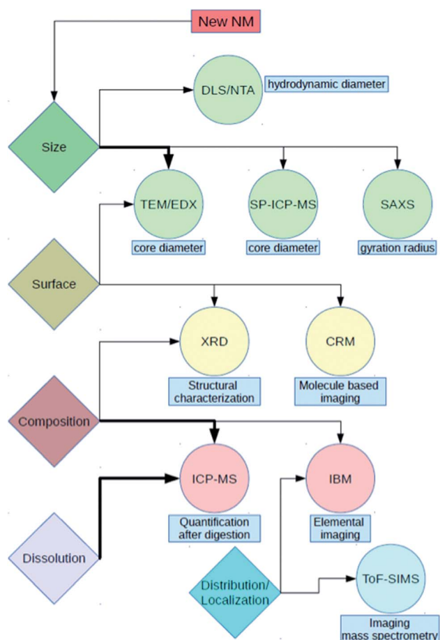
Fig. 2 Overview of key NM characteristics (colored rhombi) and methods (colored circles) used in this study for characterization. Arrows in bold imply the main method for the linked characteristic. Abbreviations: DLS – dynamic light scattering; NTA – nanoparticle tracking analysis; TEM – transmission electron microscopy; EDX – energy dispersive X-ray spectroscopy; SP-ICP-MS – single particle inductively coupled plasma mass spectrometry; SAXS – small angle X-ray scattering; XRD – X-ray diffraction; CRM – confocal Raman microscopy; ICP-MS – inductively coupled plasma mass spectrometry; IBM – ion beam microscopy; ToF-SIMS – time of flight mass spectrometry.
