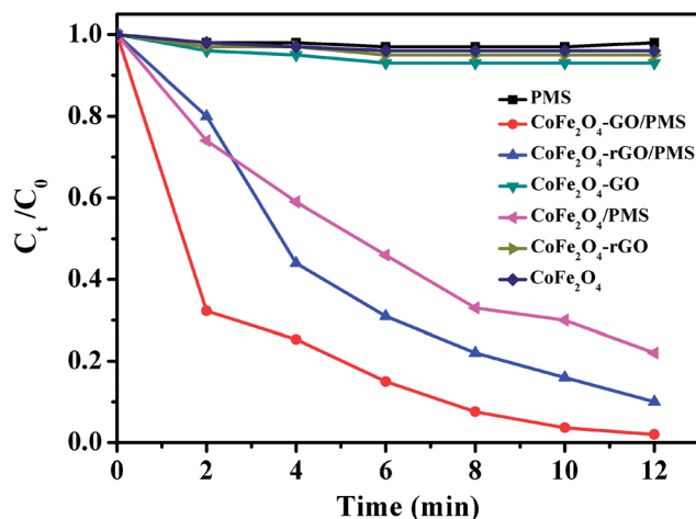
Fig. 8 RhB degradation by various catalytic PMS systems. Conditions: [\text{RhB}]_0 = 0.03 \text{ mmol L}^{-1} , [\text{PMS}] = 0.10 \text{ mg L}^{-1} , amount of catalyst = 10 mg, temperature = 25 \text{ }^\circ\text{C} .
