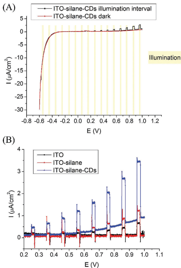
Fig. 3 (A) LSV curves of ITO-silane-CDs in the dark and with chopped illumination (420–450 nm, 10 \text{ mW cm}^{-2} , a UV blocking filter was used to block light at wavelengths < 420 \text{ nm} ); (B) LSV curves of ITO, ITO-silane, and ITO-silane-CDs with chopped illumination.
