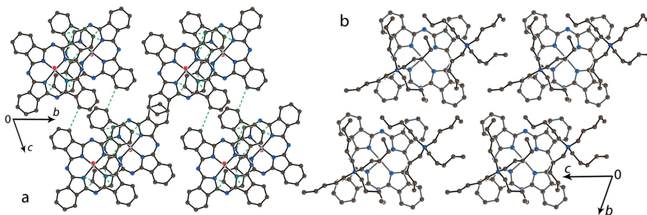
Fig. 4 (a) View of the phthalocyanine layer composed of the \pi -stacking [\text{Ti}^{\text{IV}}\text{O}(\text{Pc}^{3-})]_2^- dimers in 4 . Short van der Waals C...C, N...C, N contacts are shown by green dashed lines. (b) Projection of the \text{Pent}_4\text{N}^+ layer on the phthalocyanine layer. Only one phthalocyanine from the dimer is shown (bonds are shown in grey).
