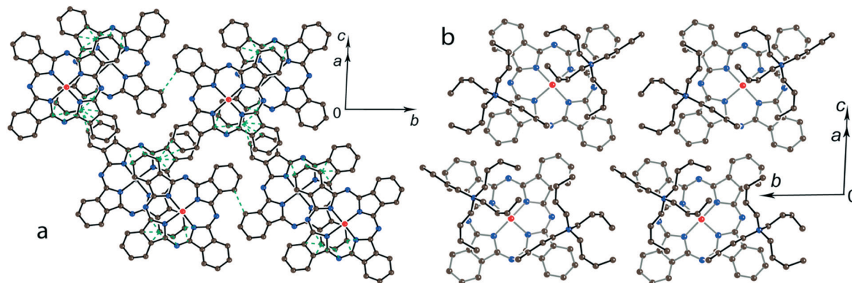
Fig. 3 (a) View of the phthalocyanine layer composed of the \pi -stacking [\text{Ti}^{\text{IV}}\text{O}(\text{Pc}^{3-})]_2^- dimers in 2 . 12 Short van der Waals C...C, N...C, N contacts are shown by green dashed lines. (b) Projection of the \text{Bu}_4\text{N}^+ layer on the phthalocyanine layer. Only one phthalocyanine from the dimer is shown (bonds are shown in grey).
