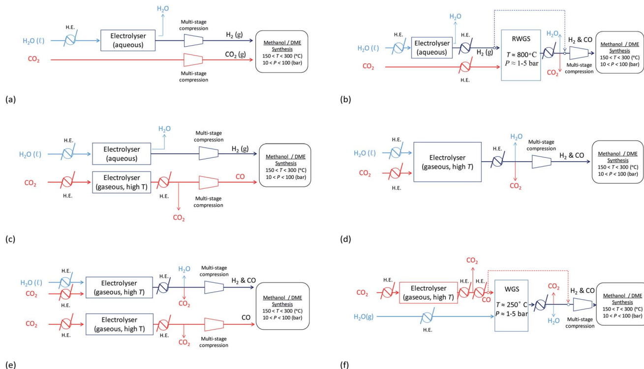
Fig. 13 Possible routes for the production of syngas, with varying ratios of \text{H}_2 : C, from \text{H}_2\text{O} and \text{CO}_2 .
