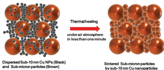
Fig. 30 Schematic illustration of the sintering mechanism of the copper-based composite inks. [Reprinted with permission from ref. 269 Copyright \text{\textcircled{C}} American Chemical Society.]
